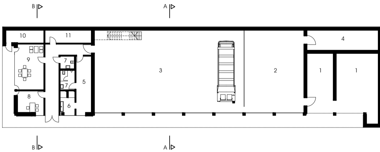
ERDGESCHOSS / PIANO TERRA
