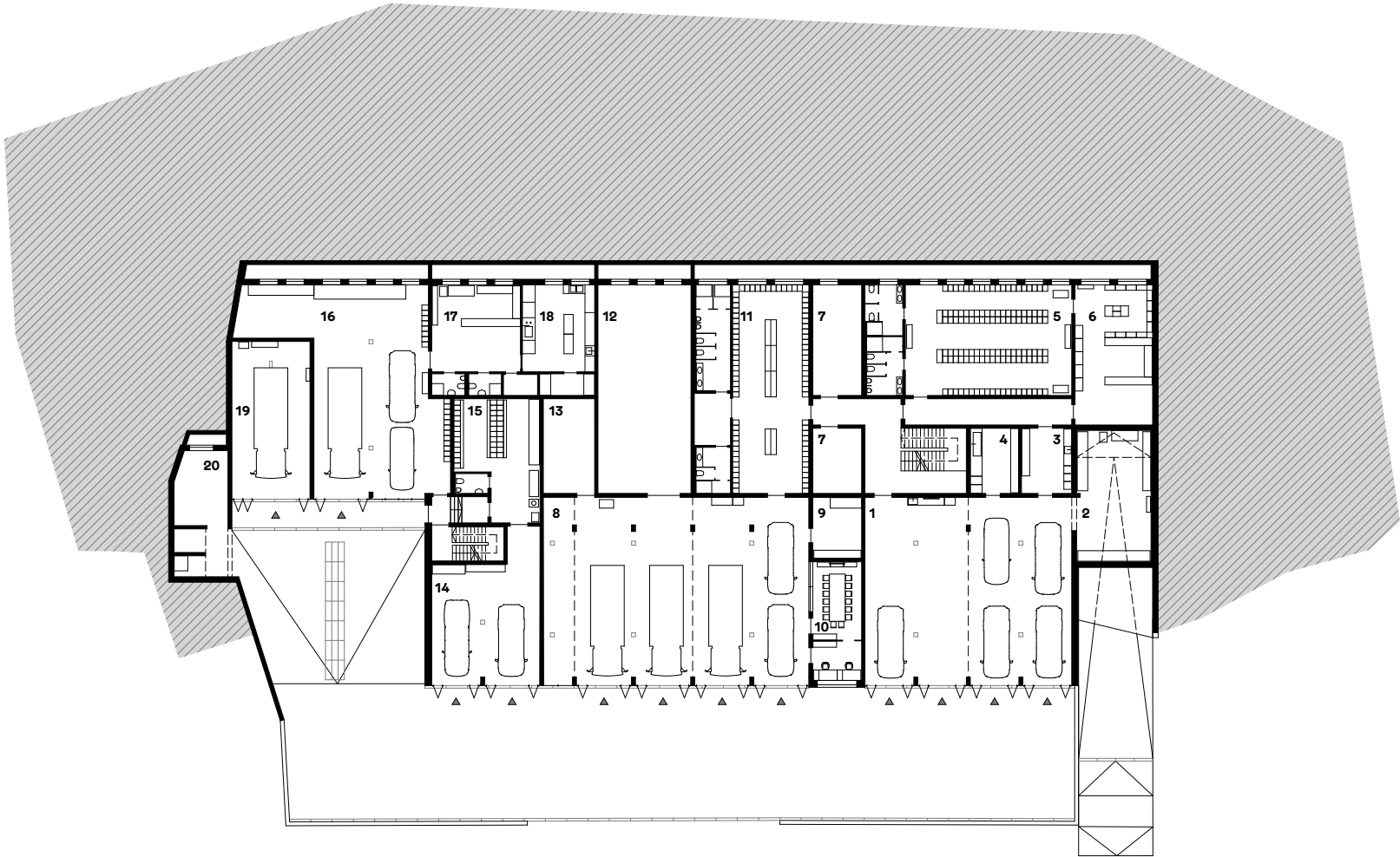
Erdgeschoss Piano terra
