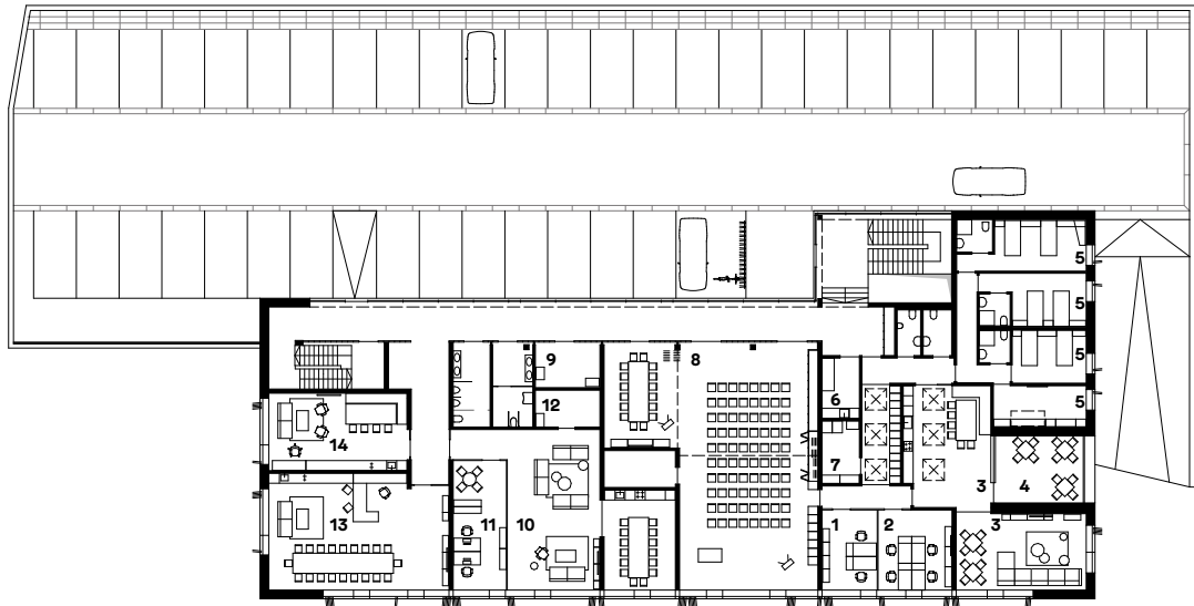
1. Obergeschoss Piano primo
