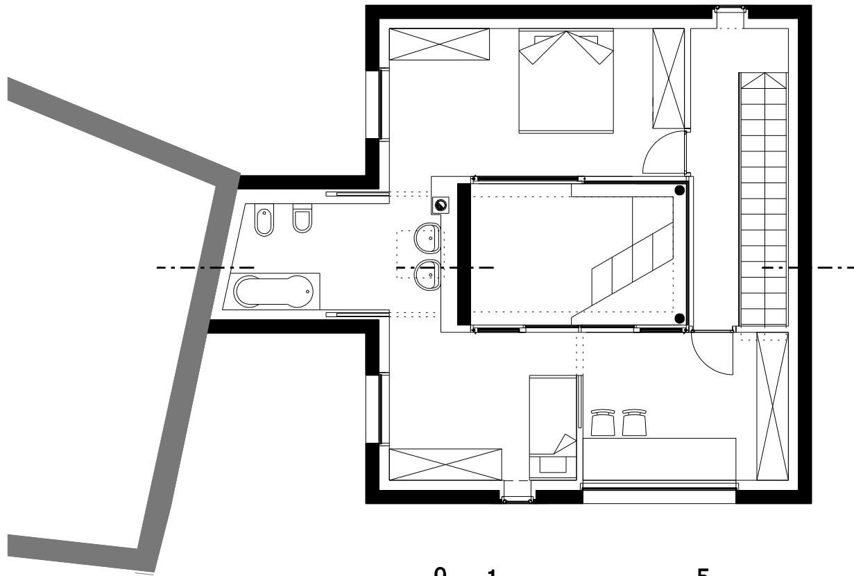
OBERGESCHOSS FIRST FLOOR
