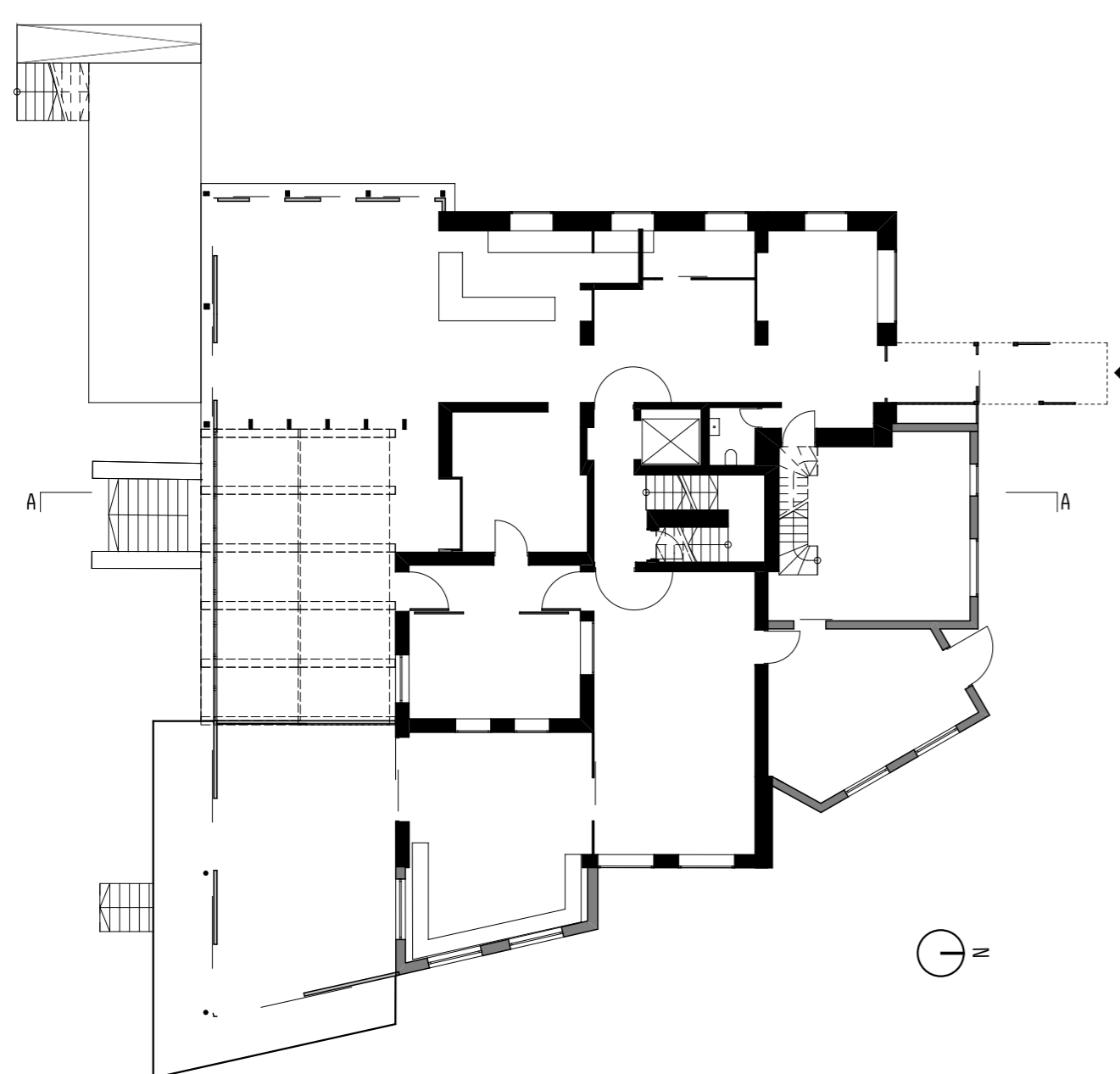
Grundriss EG Plan ground floor Pianta pianoterza
