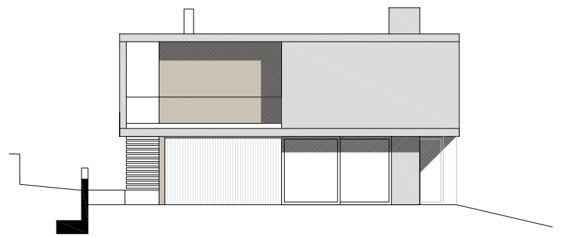
SOUTH PROSPECT
