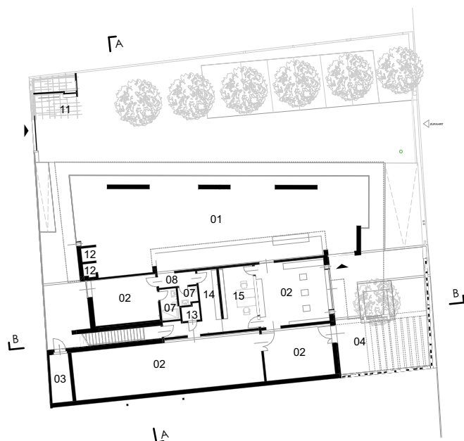
PIANO TERRA ①
