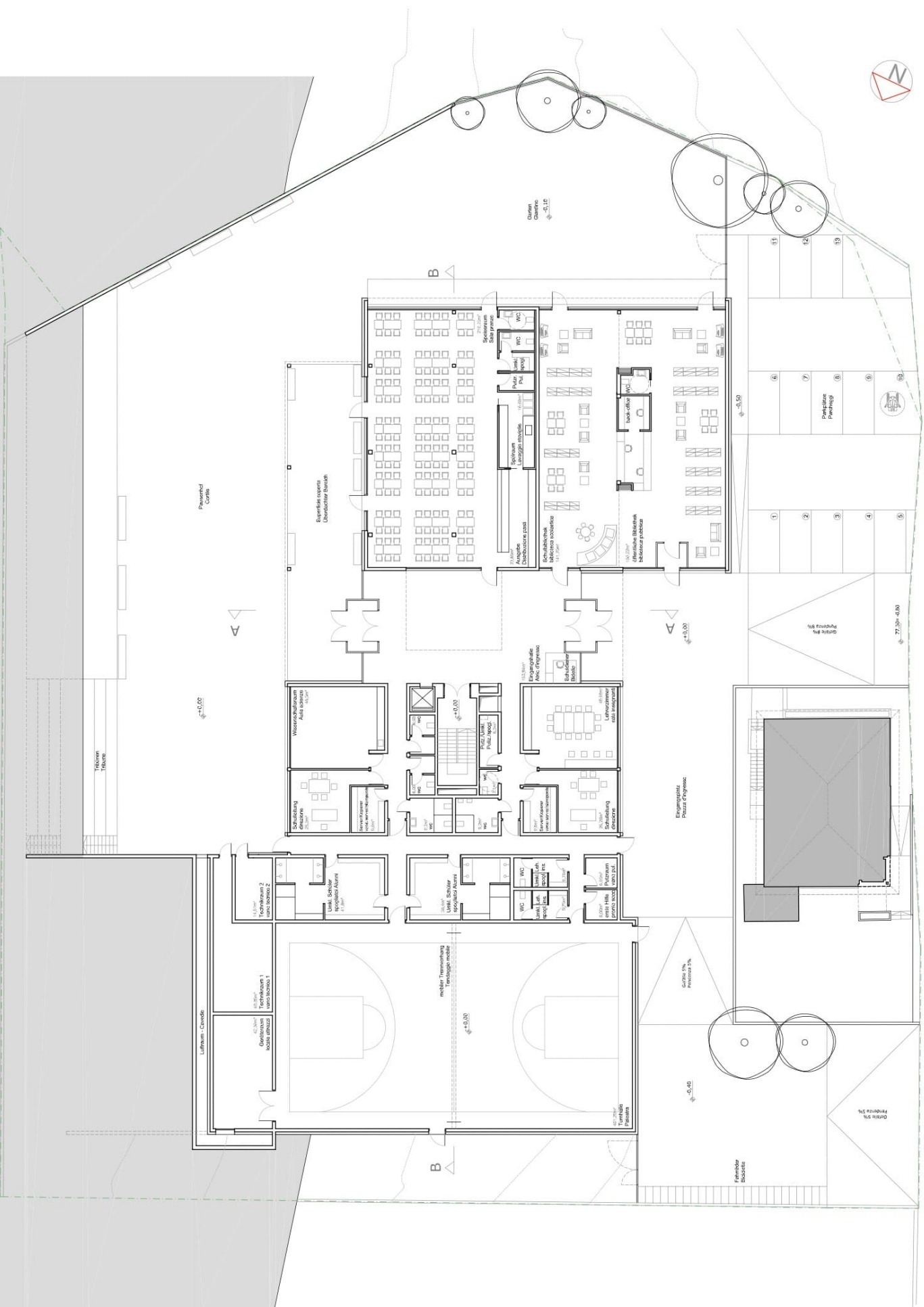
GRUNDRISS ERDGESCHOSS - PIANTA PIANO TERRA 1:200
