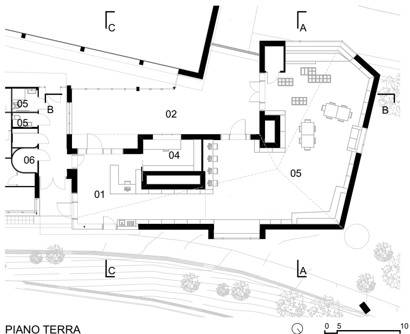
PIANO TERRA
