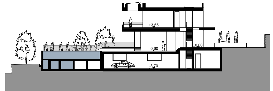
HOUSE M_SECTION B:B
