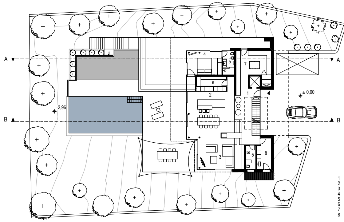
HOUSE M_GROUND FLOOR
