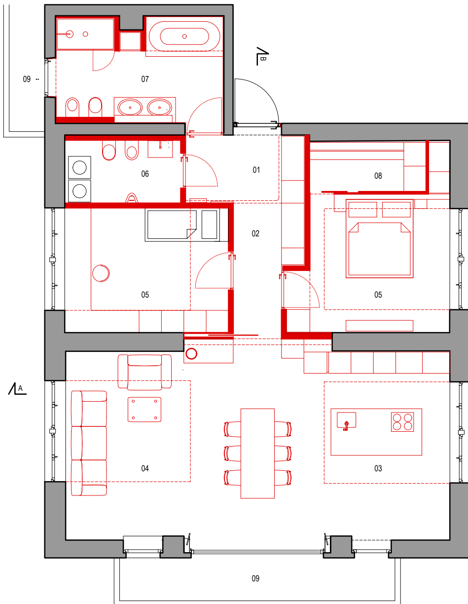
GRUNDRISS_M.1:100
