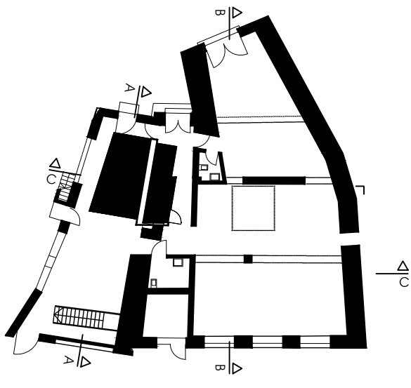
1° STOCK / PIANO
