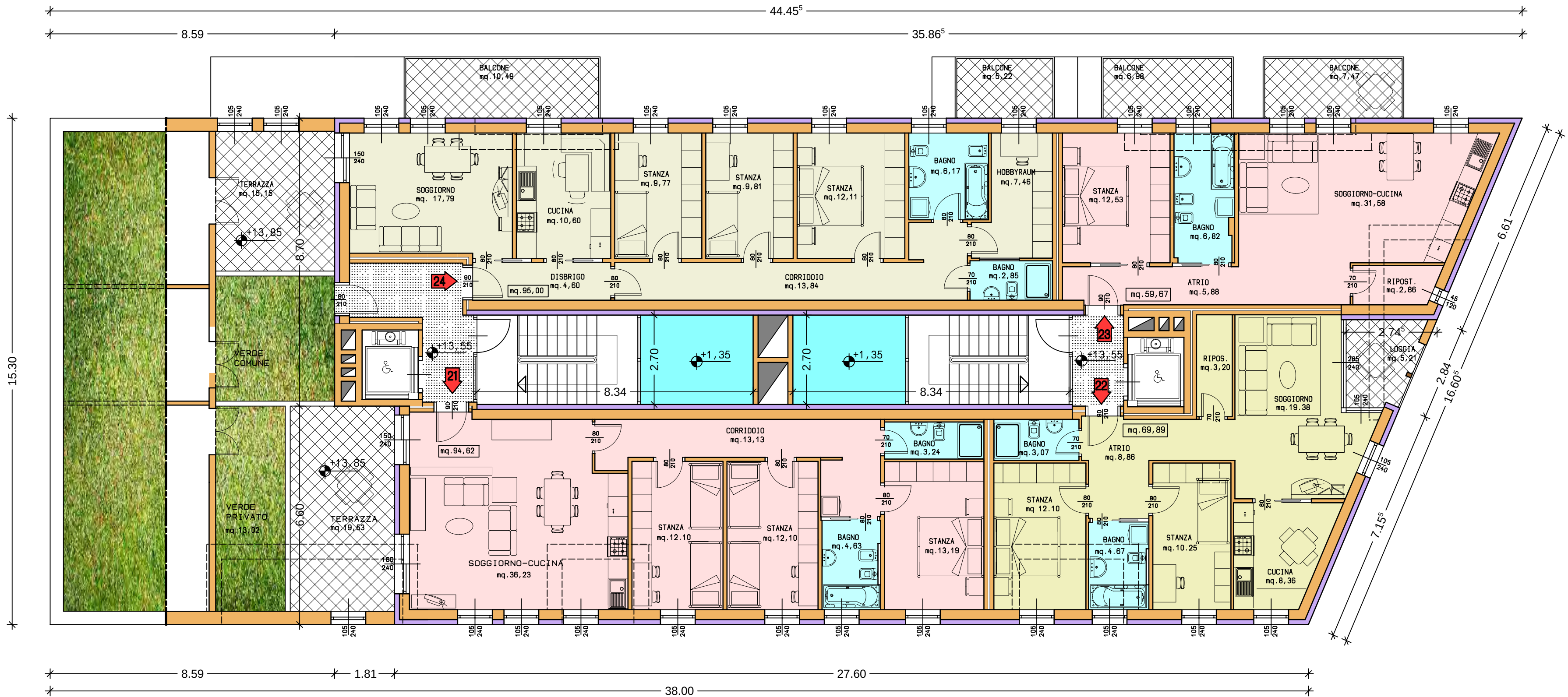
PIANO QUARTO
